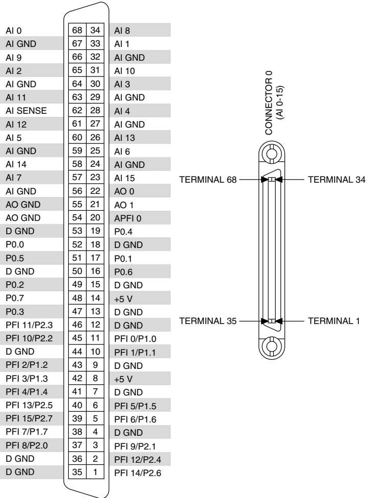
Figure 9. NI PCI/PCIe/PXI/PXIe-6251 Pinout
